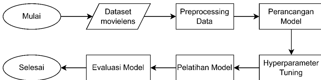
Gambar 3.1. Metode Penelitian
