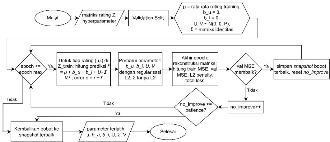
Gambar 3.5. Flowchart RSVD
